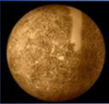
Mercury
