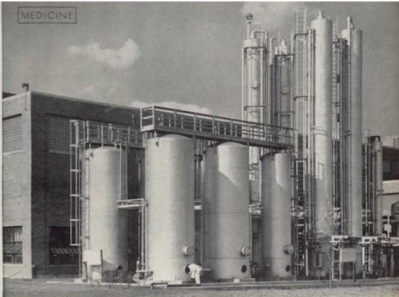
MORE TANKS AND STILLS ARE PART OF THE COMMERCIAL SOLVENTS' PENICILLIN PLANT IN TERRE HAUTE, IND. THIS IS ONE OF 10 U. S. PLANTS MASS-PRODUCING THE DRUG
