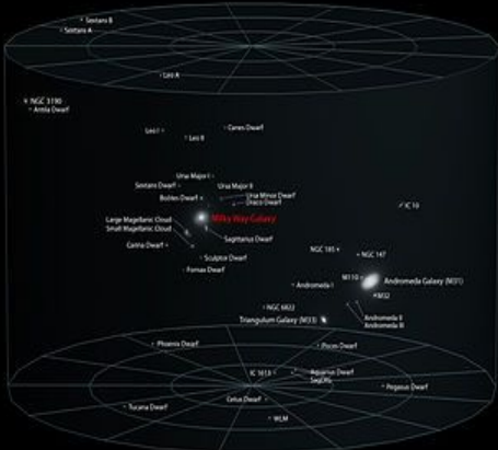
Local Galactic Group
