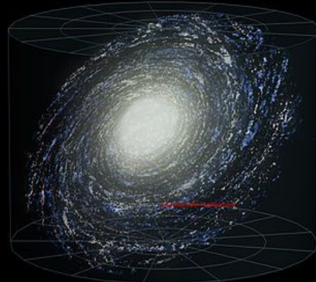
Milky Way Galaxy
