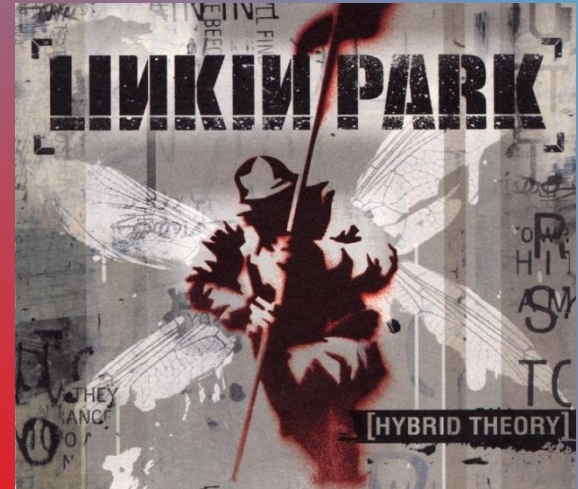
Hybrid theory
