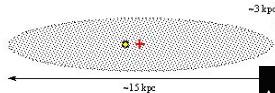
Кapteyn Model (1922)
