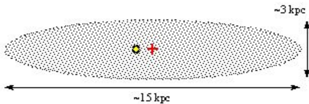
Kapteyn Model (1922)
