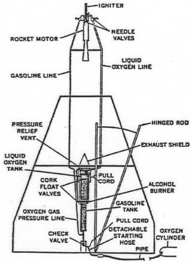
Figure 1 Dr. Goddard's 1926 Rocket
