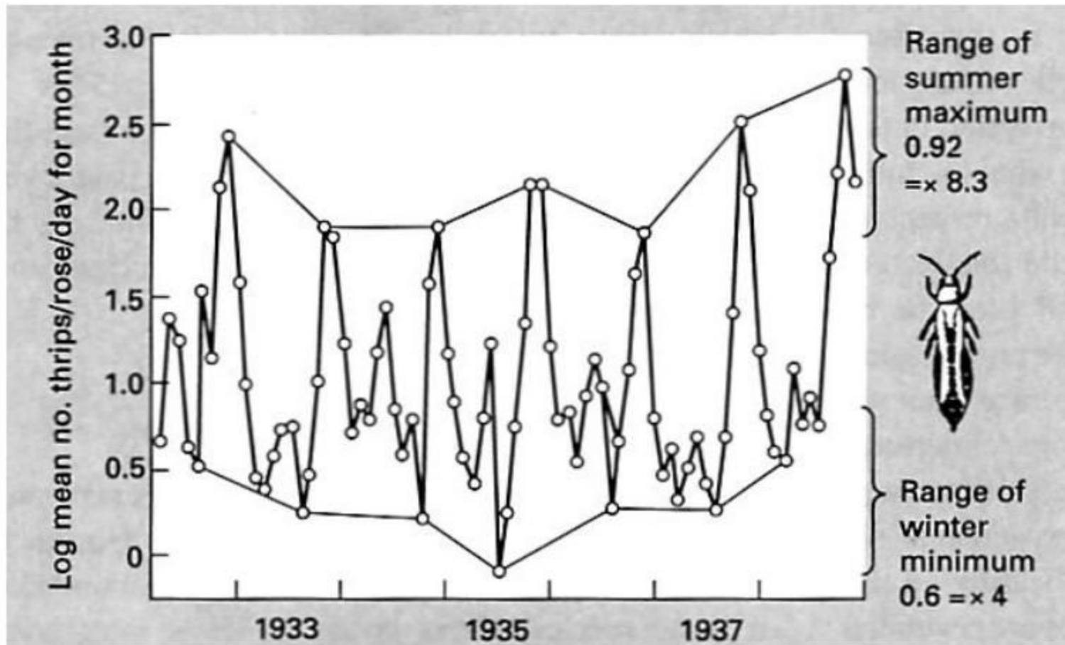
Fig. 6.1 Mean monthly population counts of adult Thrips imaginis in roses at Adelaide, Australia (Davidson & Andrewartha, 1948a) (After Varley et al. , 1975.)
