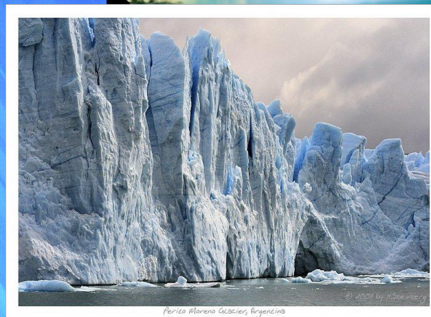
Perito Moreno Glacier, Argentina
