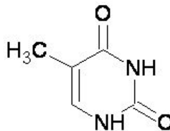
Thymine
