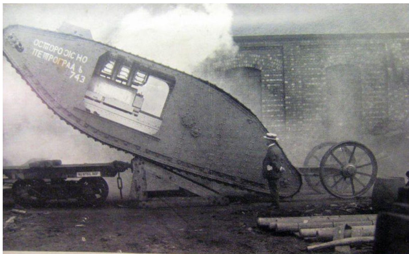
Tank mounting railway truck under own power. (p. 79)
