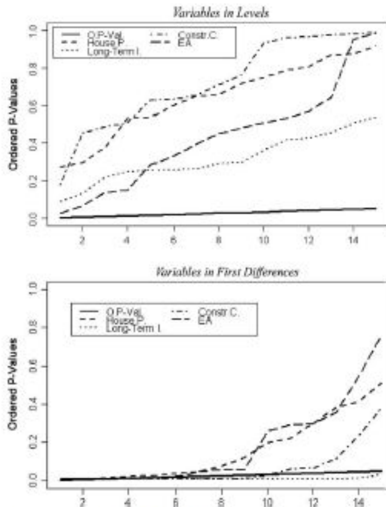
Fig. 3. Hanck panel unit root test. Calculations are based on quarterly data from 1975Q1 to 2007Q2. The null hypothesis of a unit root can be rejected if at least one ordered p-value is below the critical value of i \cdot 0.05/j for i = 1, 2, \dots, 15 , and j = 15 (thick solid line).
