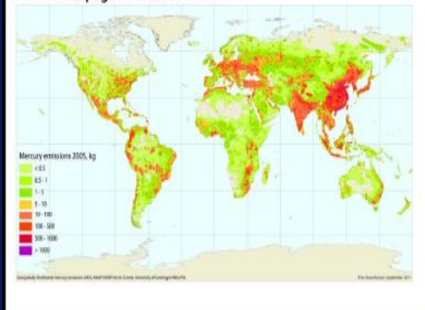
Global emissions of mercury to the atmosphere from anthropogenic sources in 2005
