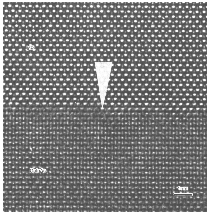
Fig. 2 \langle 110 \rangle cross-sectional lattice image of an InP/(001)GaInAs interface. Note the interfacial atomic step (arrowed). Specimen by courtesy of Dr. A.K. Petford-Long.
