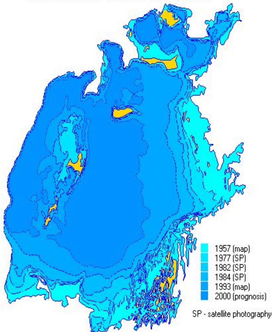
ARAL SEA AT DIFFERENT TIMES
