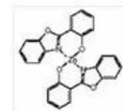
Zinc bis(2-(2-hydroxyphenyl) benzoxazolone)
