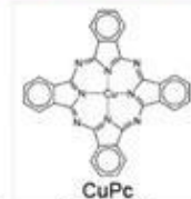
Copper(II) Phthalocyanine
