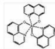
tris-(8-hydroxyquinoline) aluminum
