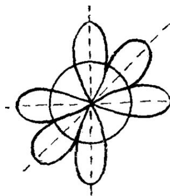
(s+p+p+p)
