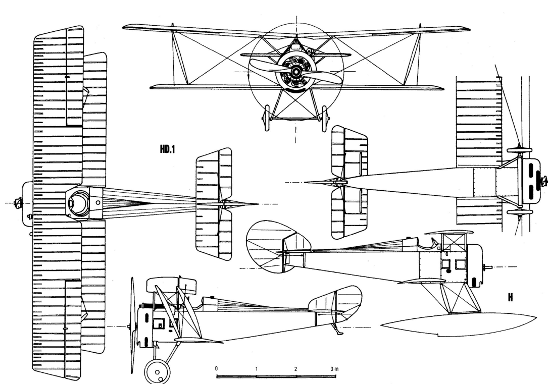
Hanriot HD.1
