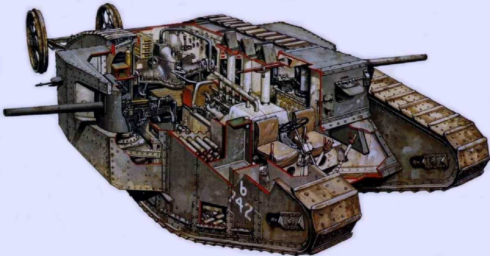
Mark I - British tank
