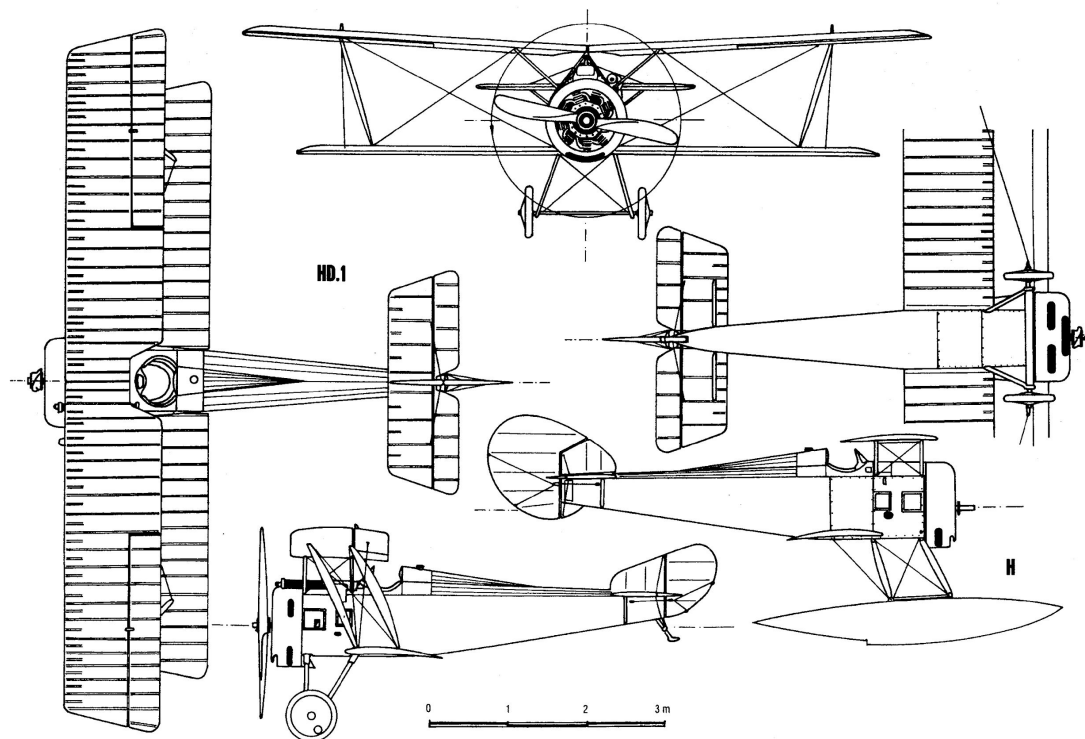
Hanriot HD.1
