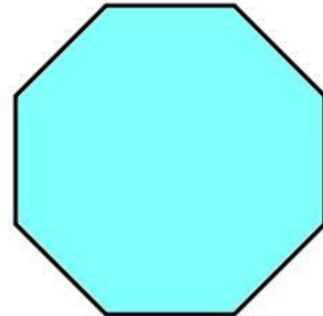
A regular octagon
