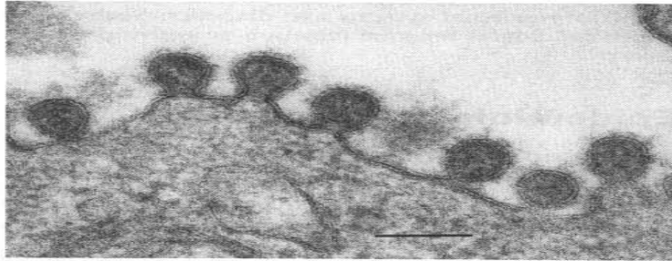
Fig. 15.18 (a) Budding influenza virus. Bar = 100 nm. (b) Spherical influenza virions budding from the surface of an infected cell. Bar = 100 nm.
