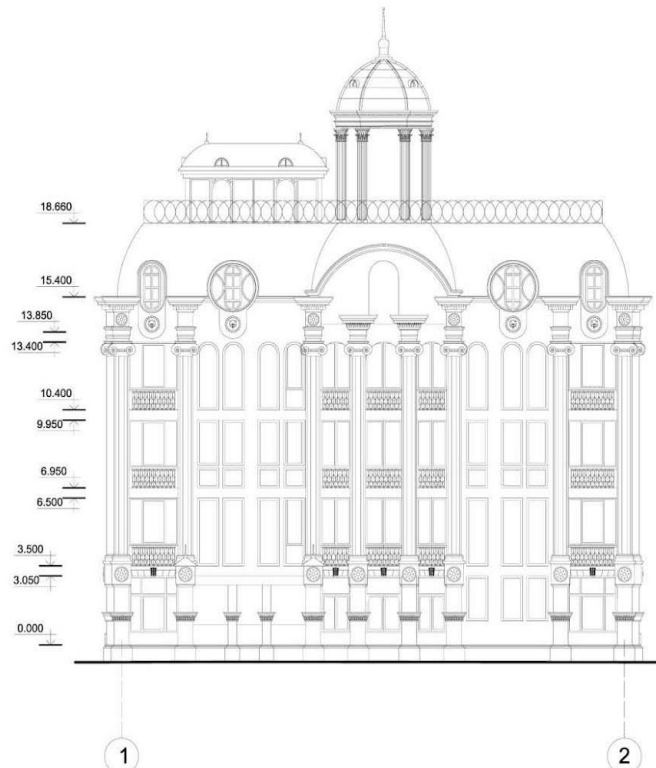
The 4-storey dwelling house (Building №2), Europolis complex, J.Omarova Str., ALMATY Chief Architect of Project - Konstantin I.Samoilov, 2004
