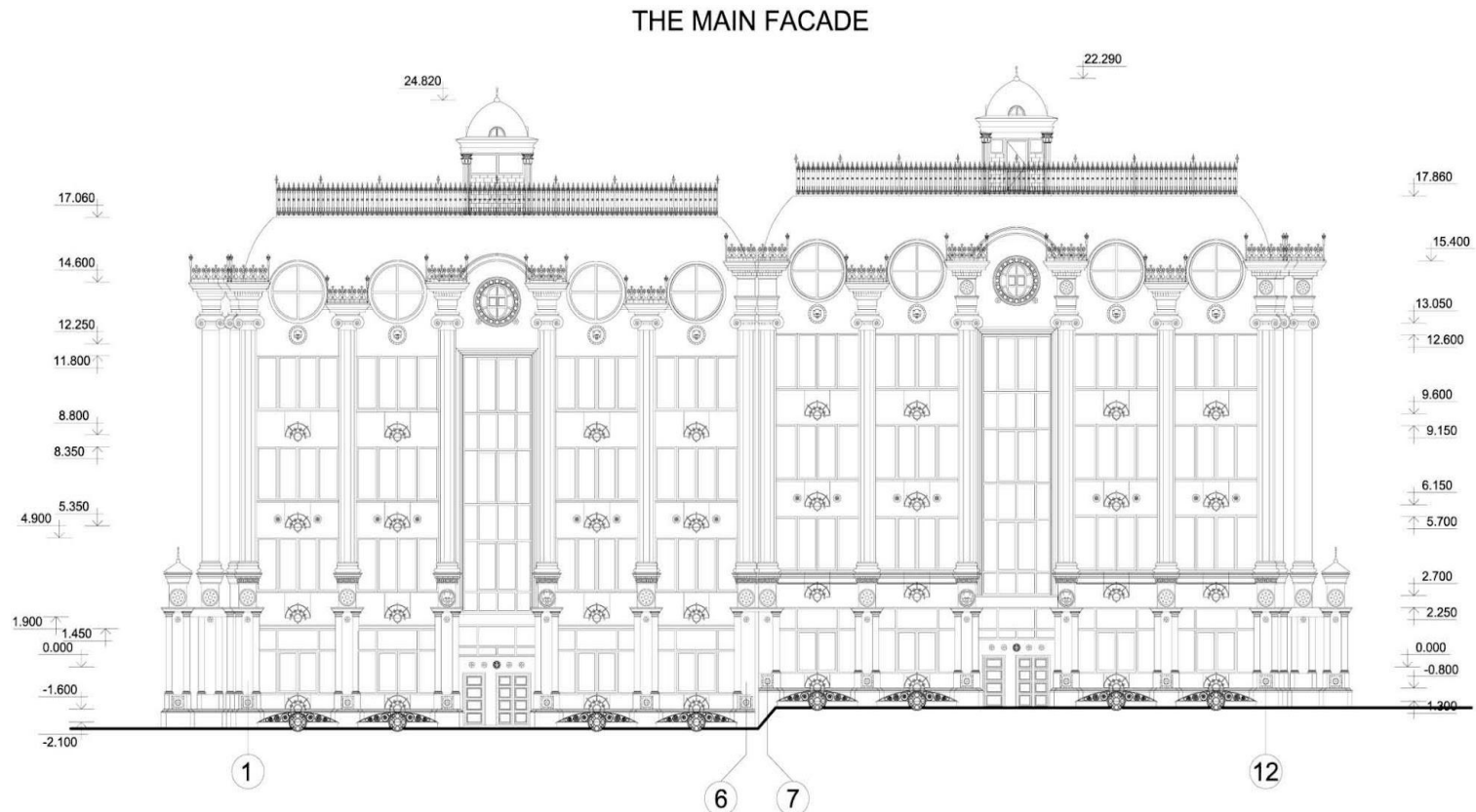
The 4-storey dwelling house (Building №5), Europolis complex, J.Omarova Str., ALMATY Chief Architect of Project - Konstantin I.Samoilov, 2005
