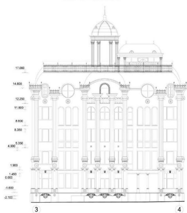
The 4-storey dwelling house (Building №3), Europolis complex, J.Omarova Str., ALMATY Chief Architect of Project - Konstantin I.Samoilov, 2005
