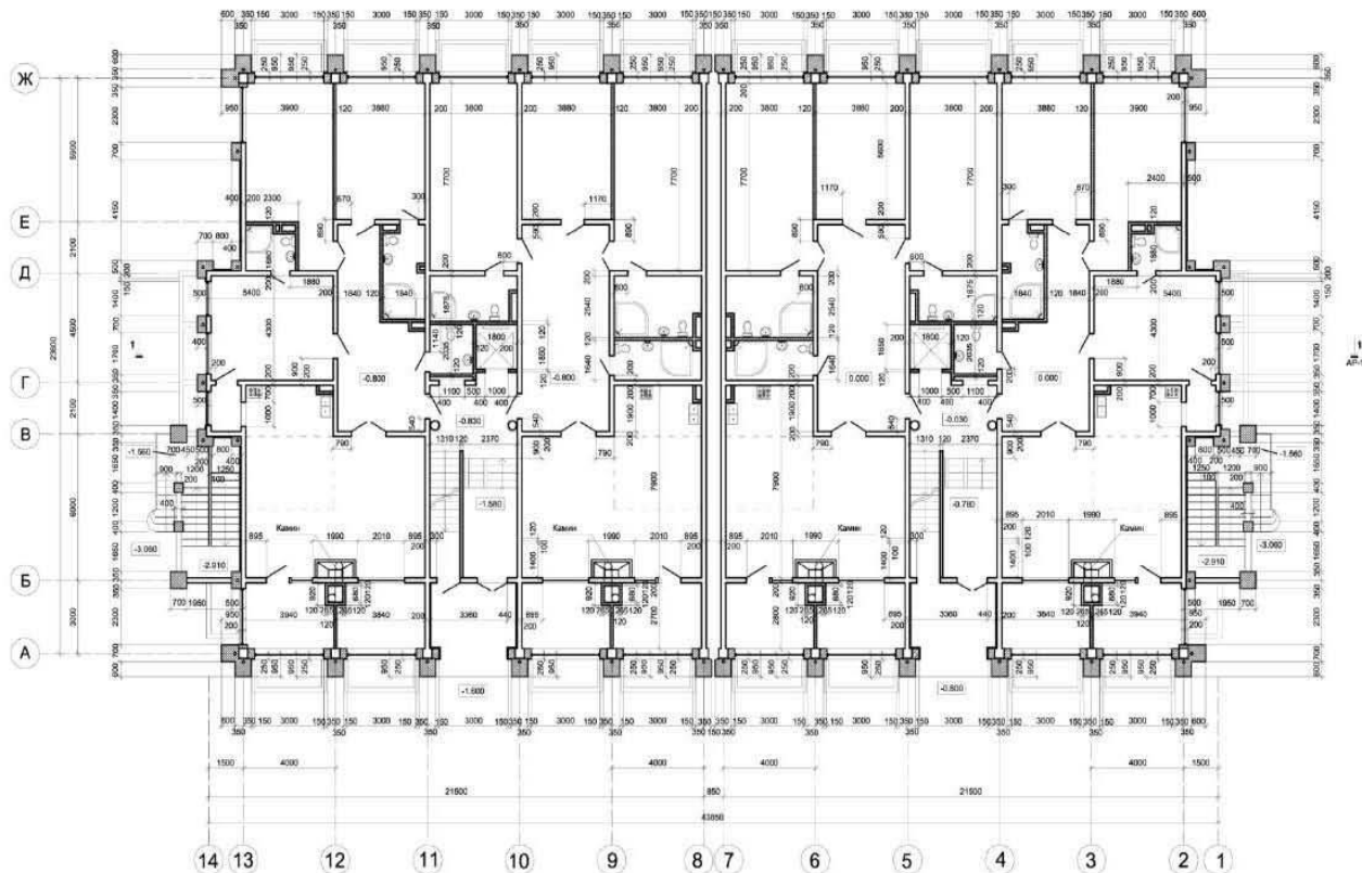
The 4-storey dwelling house (Building №5), Europolis complex, J.Omarova Str., ALMATY
