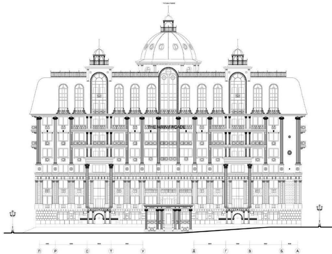
The 6-storey dwelling house (Building №7), Europolis complex, J.Omarova Str., ALMATY Chief Architect of Project - Konstantin I.Samoilov, 2007
