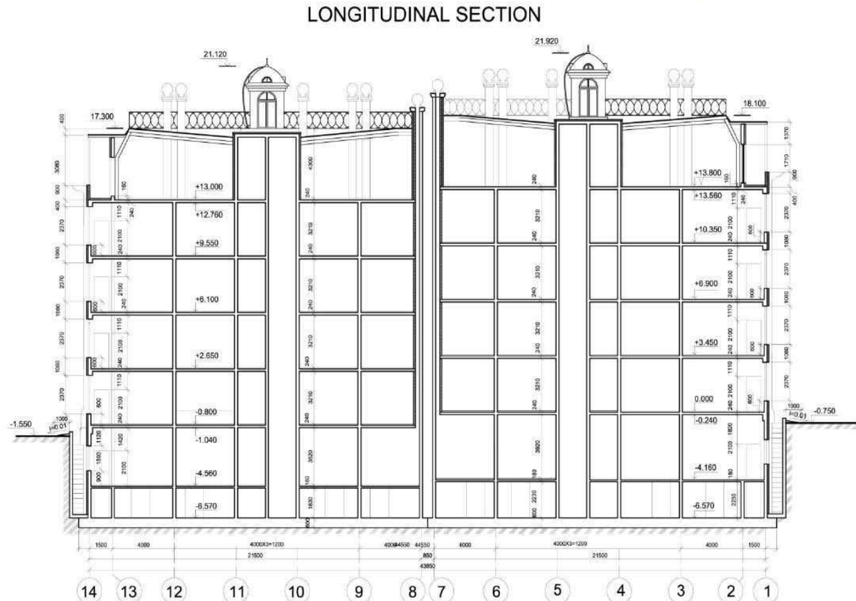
The 4-storey dwelling house (Building №5), Europolis complex, J.Omarova Str., ALMATY Chief Architect of Project - Konstantin I.Samoilov, 2005
