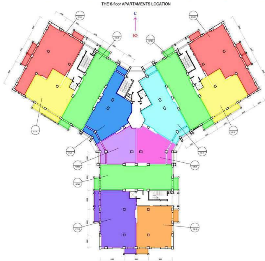
The 5-storey dwelling house (Building №7). Europolis complex, J.Omarova Str., ALMATY Chief Architect of Project - Konstantin I.Samoilov, 2006
