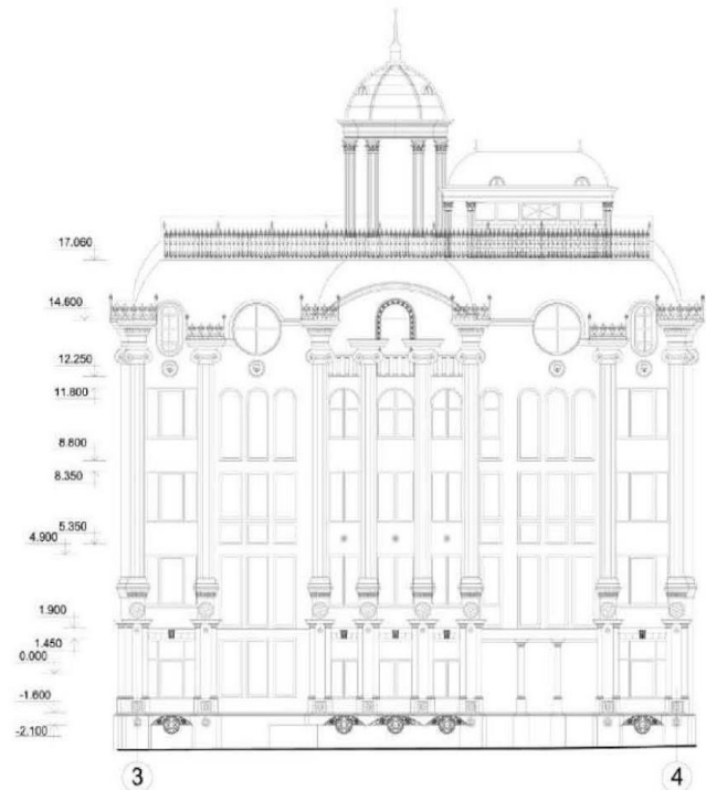
The 4-storey dwelling house (Building №3), Europolis complex, J.Omarova Str., ALMATY Chief Architect of Project - Konstantin I.Samoilov, 2005
