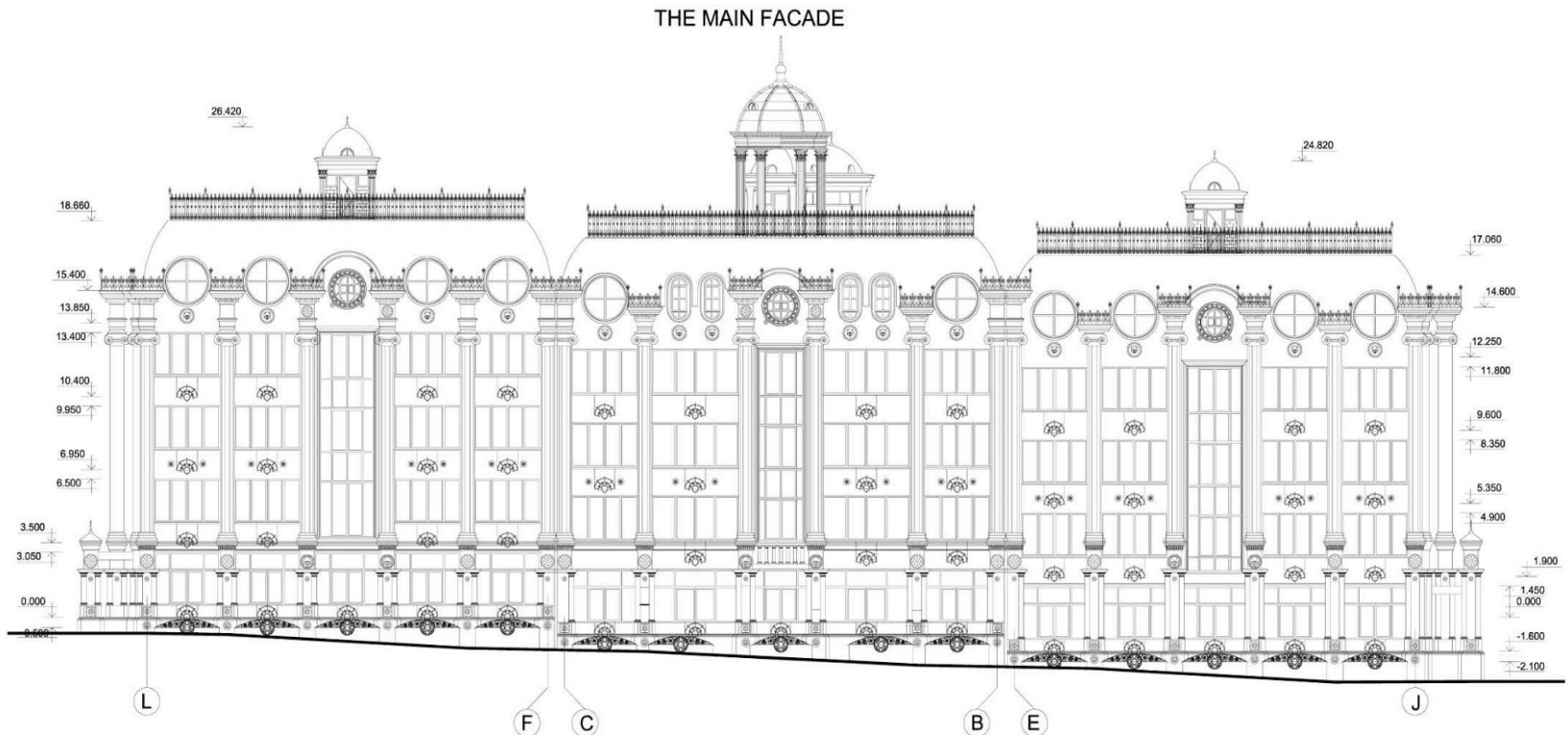
The 4-storey dwelling house (Building №3), Europolis complex, J.Omarova Str., ALMATY Chief Architect of Project - Konstantin I.Samoilov, 2005
