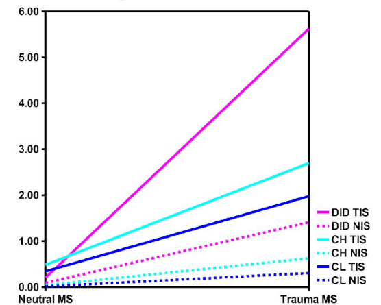
Emotional rating
