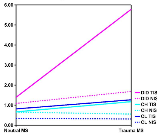
Sensori-motor rating
