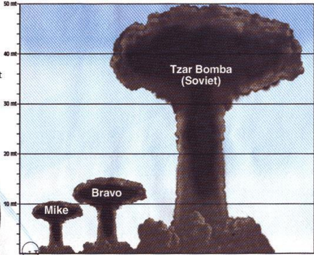
Comparison of explosive yeilds for nuclear weapon tests.
