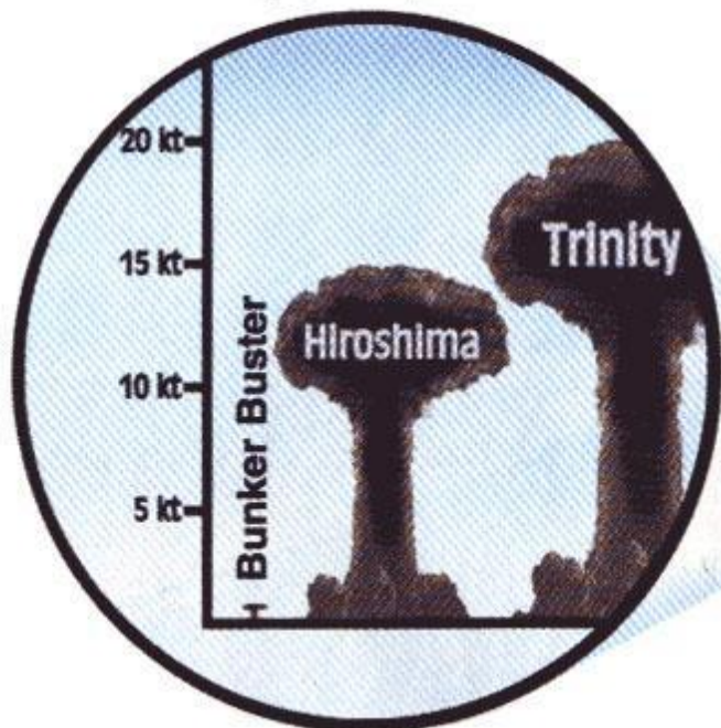
Comparison of explosive yeilds for nuclear weapon tests.
