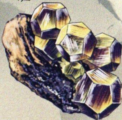
Pyrite
