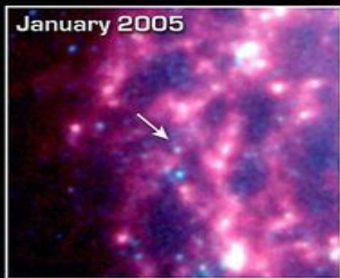
Supernova Dust Factory in Galaxy M74 NASA / JPL-Caltech / Ben E. K. Sugerman (STScI)
