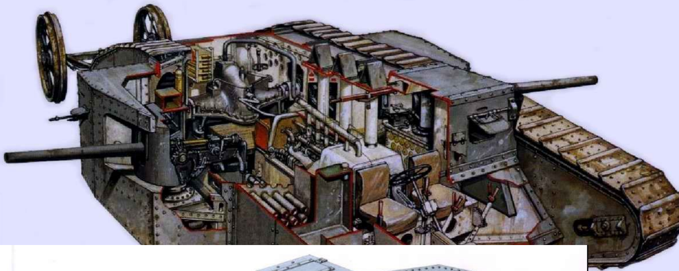
Mark I - British tank
