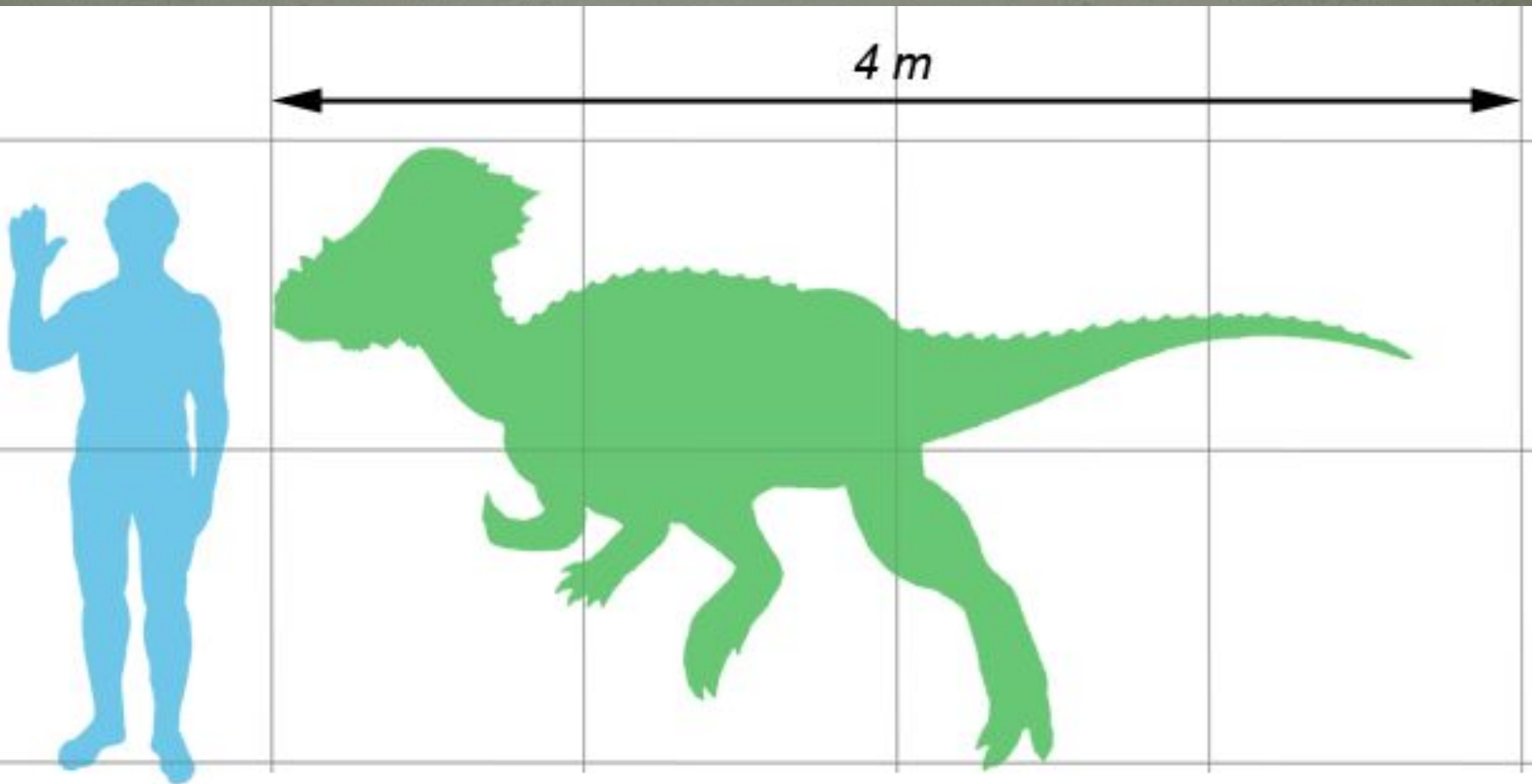
Pachycephalosaurus wyomingensis
