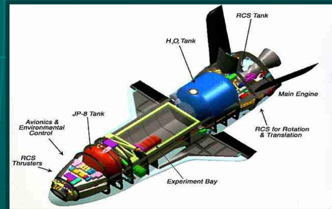
X-37 B
